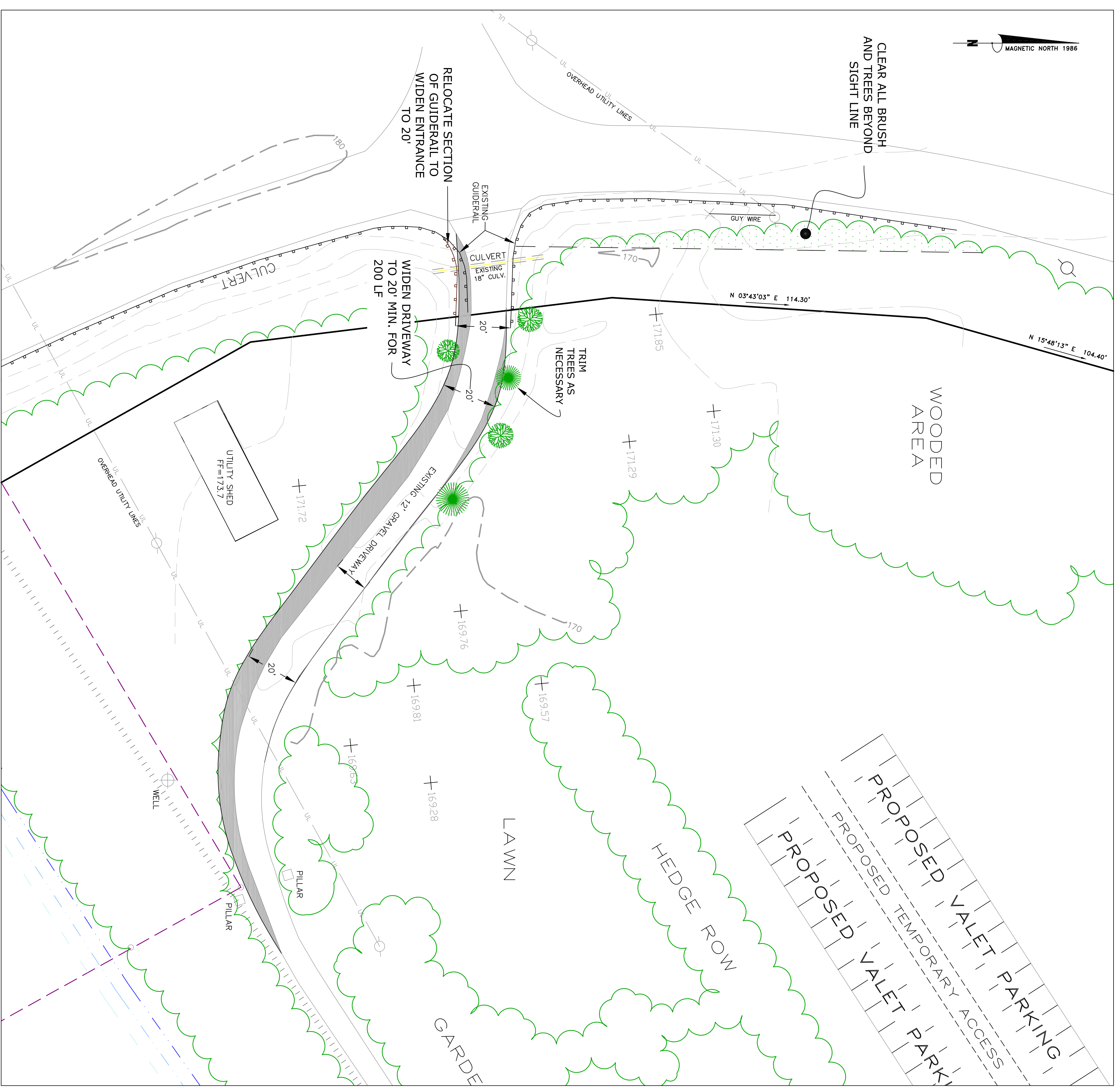
DRIVEWAY IMPROVEMENT-PLAN VIEW SCALE: 1"=20' Base elevation from USGS topographic maps.
